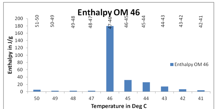
Temp Vs Enthalpy data for PCM OM46P
