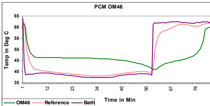
T-History graph PCM OM46P
